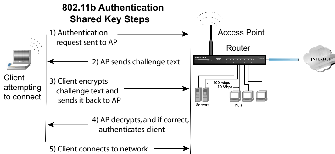
Figure D-2: 802.11b shared key authentication
