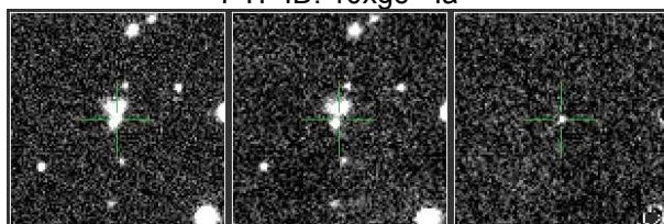
PTF ID: 10xjm - Ia
