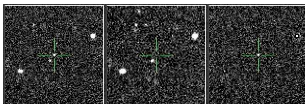
PTF ID: 10absf - II
