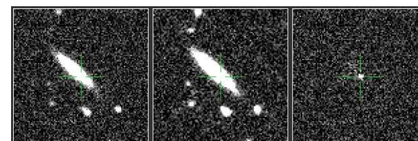
PTF ID: 10rin - II
