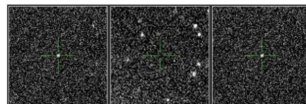
PTF ID: 10weh - IIa
