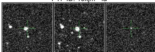
PTF ID: 10yad - Ia
