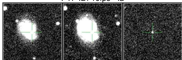
PTF ID: 10ksq - IIP
