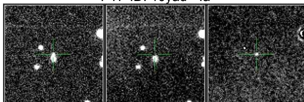
PTF ID: 10ydz - Ia
