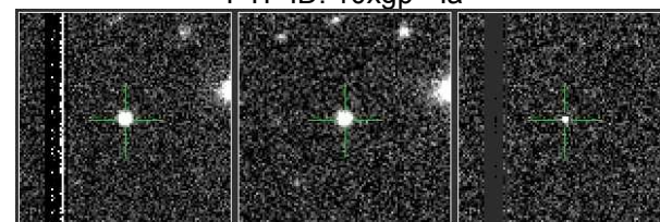
PTF ID: 10xla - Ib/c
