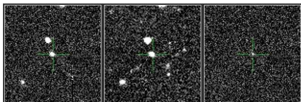
PTF ID: 10zhi - Ia
