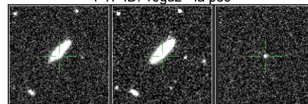
PTF ID: 10myz - IIP
