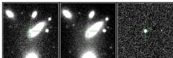
PTF ID: 10fps - Ia
