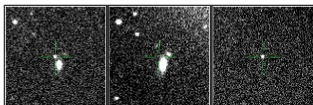
PTF ID: 10vyl - Ia
