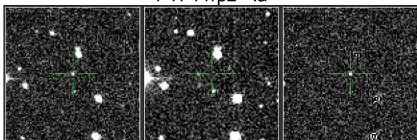
PTF11ncy - Ia
