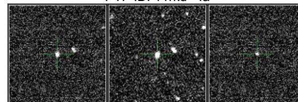
PTF11ms - Ia
