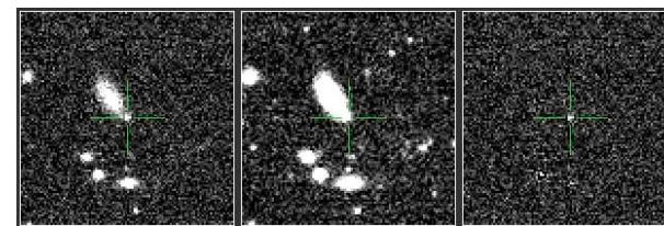
PTF12dke - II
