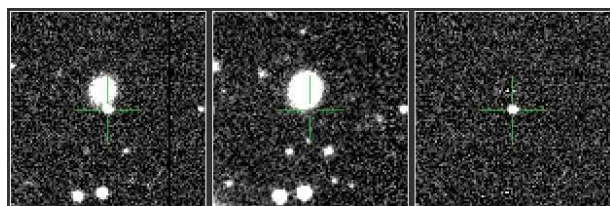
PTF12ccz - Ia
