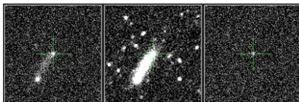
PTF12cde - Ib/c
