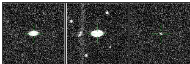
PTF12dwm - Ia
