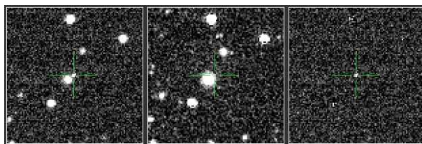
PTF12dgy - Ia
