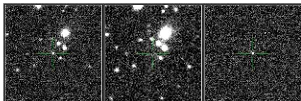
PTF12cdd - Ia
