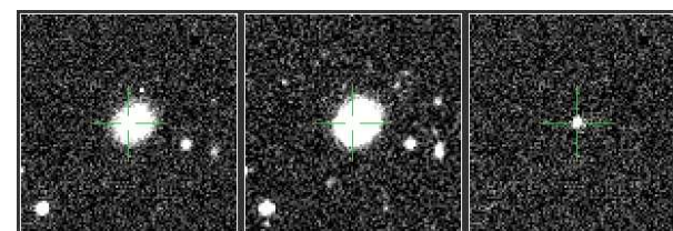
PTF12awi - Ia
