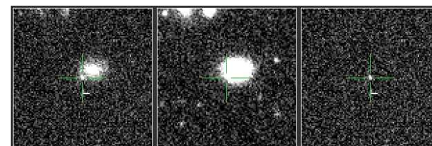
PTF12cdc - II
