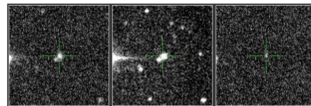
PTF12bwc - Ia
