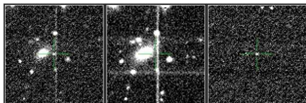
PTF12dsu - Ia
